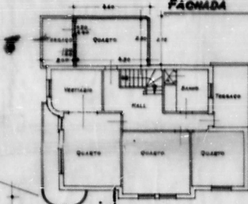
PAV. SUP. 1:100
