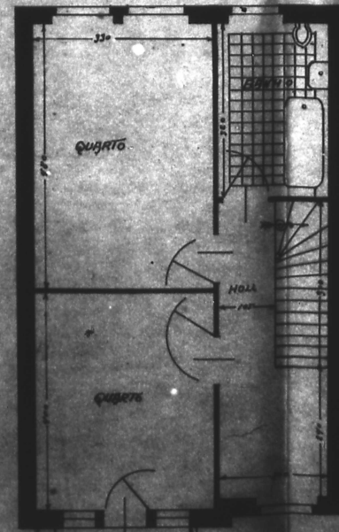
— PLANO SUPERIOR —
